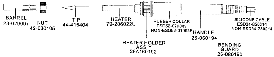
SOLDERING IRON ASSEMBLY 207/207ESD
