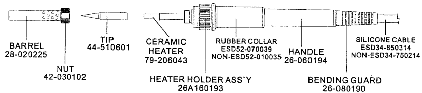
SOLDERING IRON ASS'Y 107/107ESD
