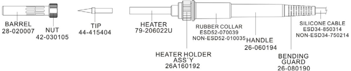
Fig. 1 SOLDERING IRON ASS-Y 207/207ESD
